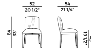
840 sedia \ chair
